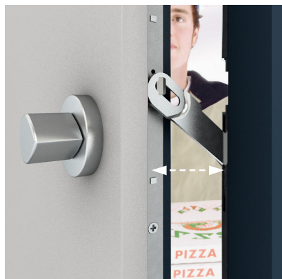
... limits the door opening to gap width – wide enough to talk to the person outside, but not wide enough to allow entry.
